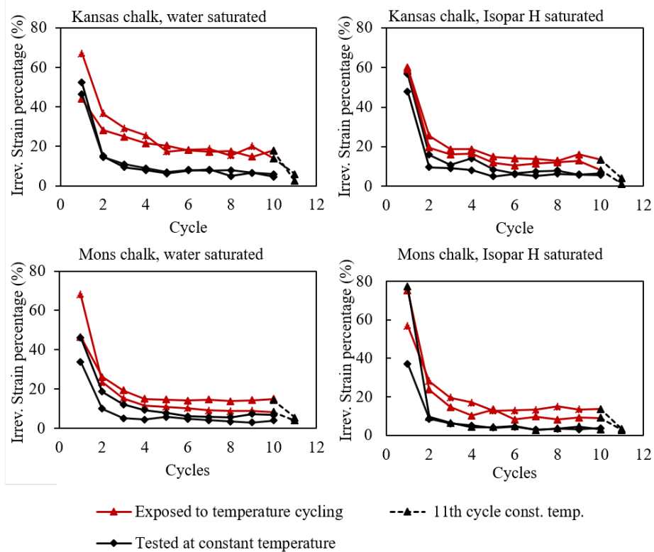
Figure 19- Irreversible strain for individual stress cycles. The red lines illustrate the test results for samples that have been exposed to temperature cycling, and black lines the samples tested at a constant temperature. The dashed line represents the result for the 11th cycle, which was only performed on samples exposed to temperature cycling. This cycle did not include a temperature cycle.
