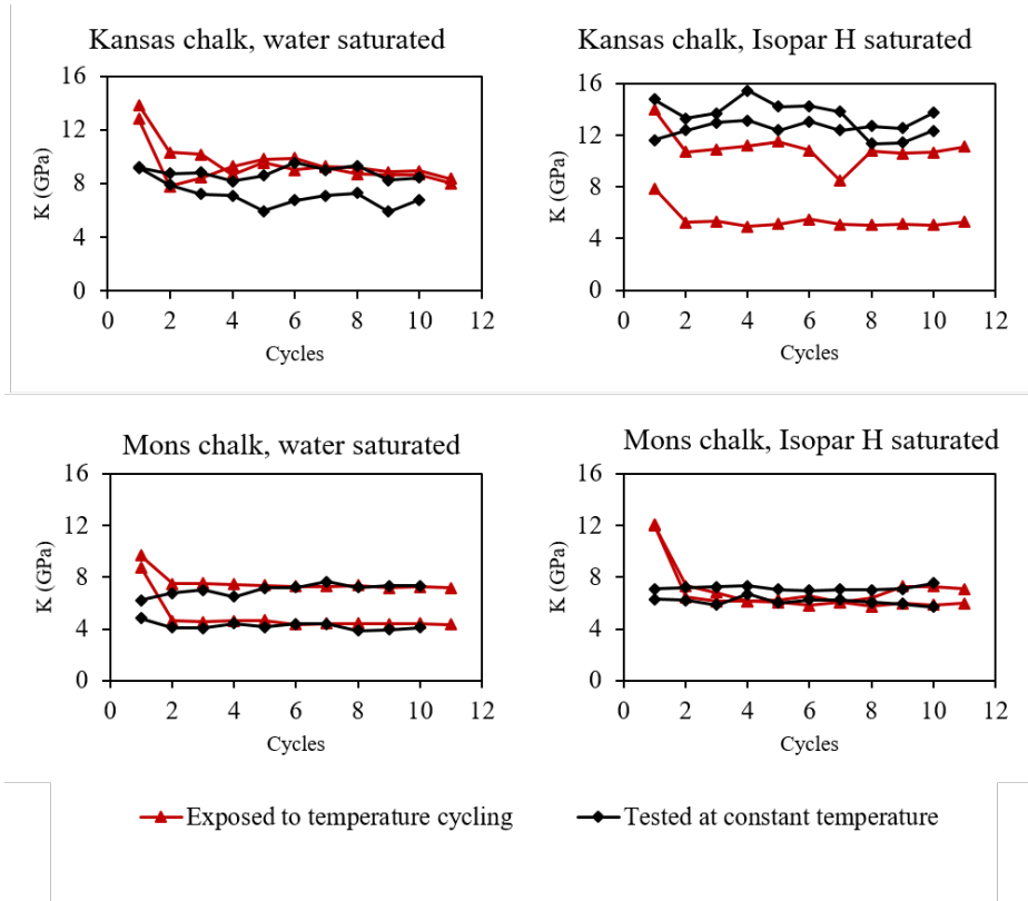
Figure 16 - Elastic bulk modulus K through a number of hydrostatic stress cycles. Red lines represent samples exposed to temperature variation between each stress cycle, and black lines correspond to samples held at a constant temperature.
