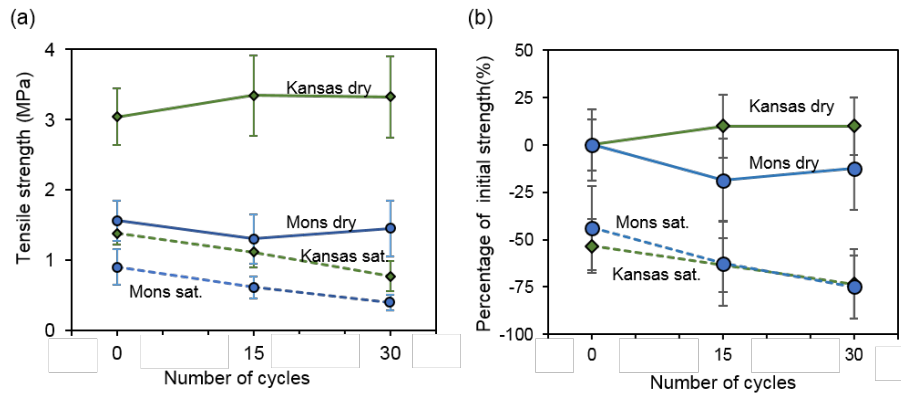
Figure 14 - (a) Average tensile strength and standard deviation as a function of number of temperature cycles in absolute measurements. (b) Tensile strength difference (in percent) as function of temperature cycling, reference is the dry and 0 cycles for each chalk type.
