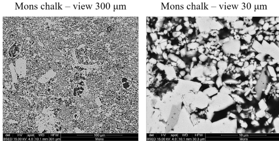
Figure 8 - Backscatter electronic micrographs of Mons chalk with two magnifications
