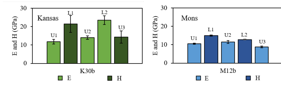
Figure 22 - Young's modulus E (lighter colour) and uniaxial compression modulus H (darker colour) measured during unloading (U) and loading (L) under constant overburden experiments.
