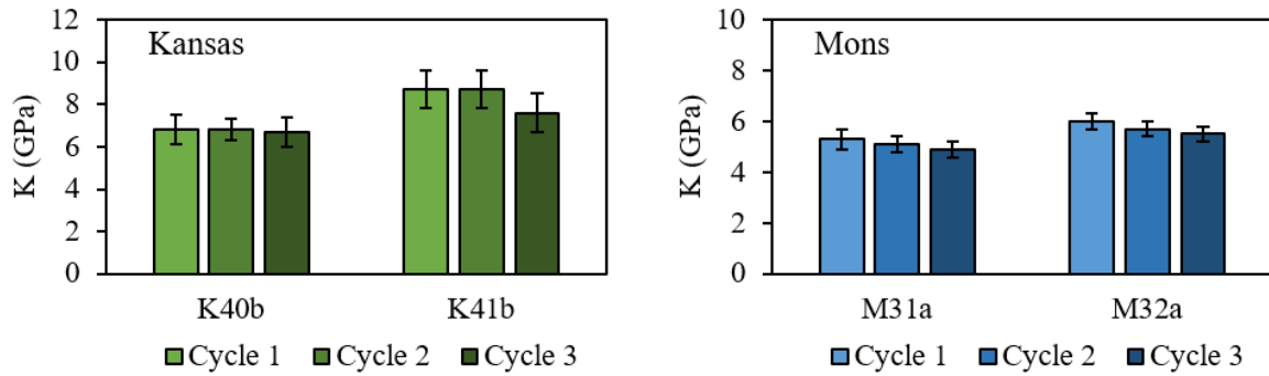
314 Figure 6. Elastic bulk modulus K estimated from hydrostatic stress reduction. The light color 315 represents the first stress unloading which is followed by temperature cycling, the intermediate 316 color second stress unloading, and the dark color represents the third stress unloading.
