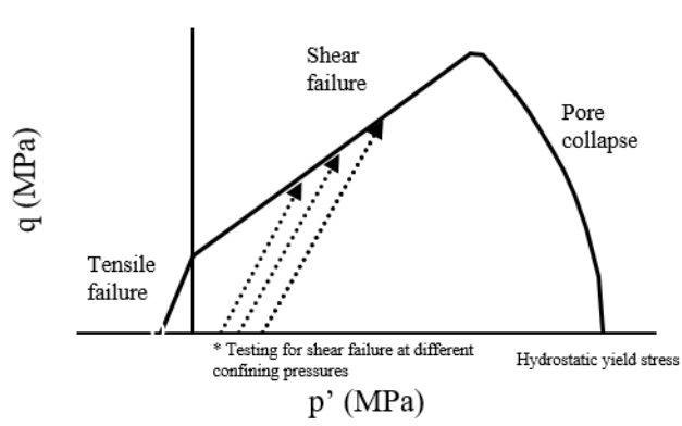
Figure 6 – p' – q diagram indicating different modes of failure. The arrows represent the direction of deviatoric loading at different confining pressures until shear failure line is reached and the sample fails.
