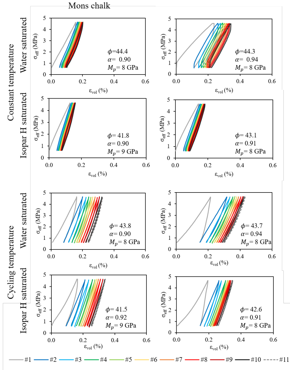
Figure 18 - Stress-strain curves for 10 or 11 cycles for Mons chalk tested at constant temperature (top two rows) and with a temperature cycle in between stress cycles (bottom two rows).
