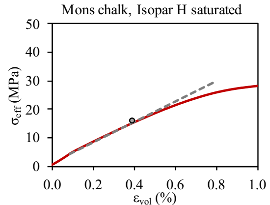
Fig. 5. Yield stress was determined when the stress difference between the measured stress–strain curve and the linear-elastic line exceeded 0.25 MPa.
